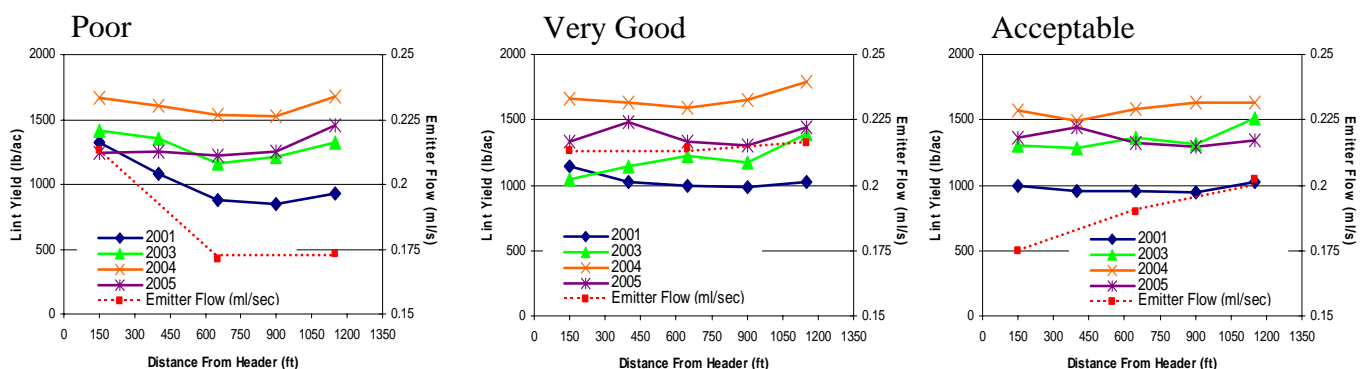
Fig. 1. Comparison of 2001, 2003, 2004 and 2005 cotton lint yields to SDI emitter flow rates at multiple locations along drip laterals of three drip uniformity designs.
